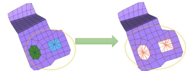
OUTPUT: The Parts are replaced, Bolt Connections are modified and Solver is changed into Nastran for Output model
