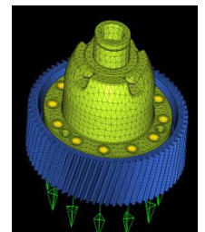
OUTPUT: The Parts are replaced, Bolt Connections are modified and Solver is changed into Nastran for Output model
