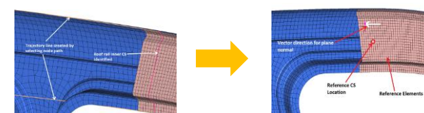
BSO Inner Part Creation
